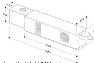
Laser Head Model D300+ 14
