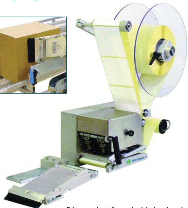
Printer and applicator in right hand version
